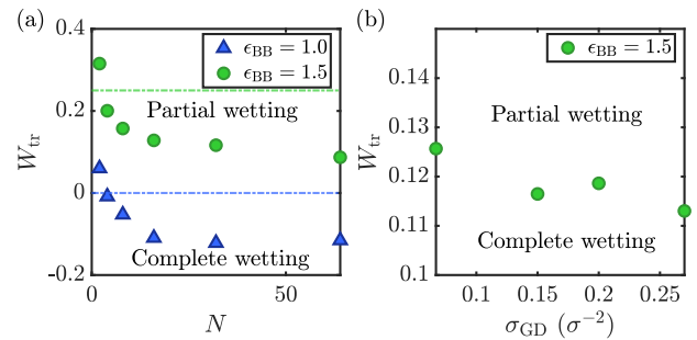
Fig. 6 The interaction parameter transition points W_{\text{tr}} , for complete to partial wetting, are plotted as (a) a function of the melt chain length N , and (b) the grafting density \sigma_{\text{GD}} . The wetting transitions based on an enthalpic estimate are given as the blue and green dash-dotted lines, for \epsilon_{\text{BB}} = 1.0 and \epsilon_{\text{BB}} = 1.5 , respectively.
