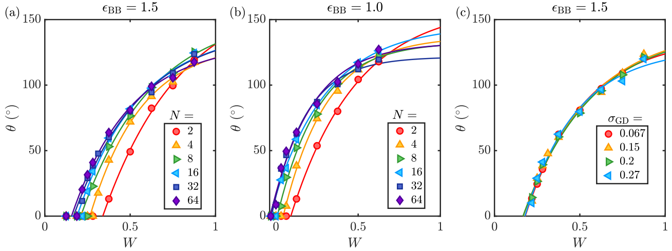
Fig. 5 Contact angle measurements for varying degrees of the interaction parameter W . (a) Shows the contact angles \theta for a brush wetted by a melt of varying degrees of polymerization N , at \epsilon_{\text{BB}} = 1.5 and \sigma_{\text{GD}} = 0.15 . (b) Shows the contact angles of varying melt chain lengths at \epsilon_{\text{BB}} = 1.0 and \sigma_{\text{GD}} = 0.15 . (c) Depicts the influence of the brush grafting density \sigma_{\text{GD}} on the contact angles for N = 32 .
