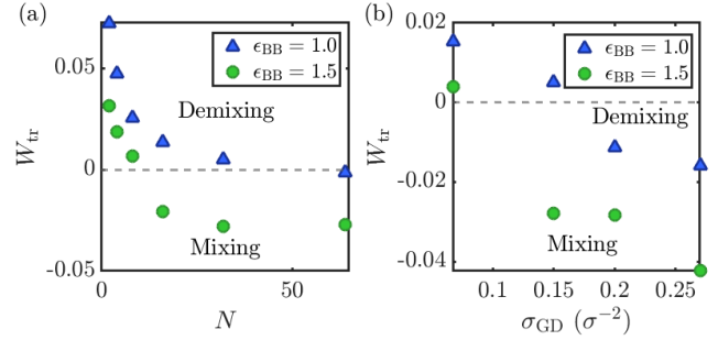
Fig. 4 The interaction parameters W_{\text{tr}} at which the mixing to demixing transition occurs, as measured from the overlap integral, (a) for a defined melt length N , and (b) grafting density \sigma_{\text{GD}} . The gray dashed lines in both figures describe the transition using predictions based on enthalpic arguments alone.
