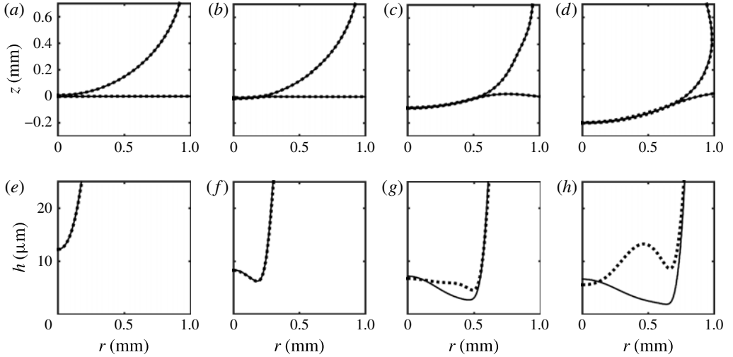
FIGURE 8. Drop impact onto a liquid pool: (a,e) t = 0.30 , (b,f) t = 0.50 , (c,g) t = 1.50 , (d,h) t = 3.00 ms. The impact speed is U = 0.14 m s ^{-1} and the drop radius is R = 0.95 mm. The density and surface tension of the liquid are respectively \rho = 916 kg m ^{-3} and \gamma = 0.020 N m ^{-1} . These impact parameters correspond to St = 6.7 \times 10^3 and We = 0.85 . (a–d) The macroscopic droplet shape together with the pool shape is shown. The solid line corresponds to calculations made in the moving (n, s) -coordinate system. The dashed line shows the result for the same case with the only difference being that lubrication is now calculated in a conventional (r, z) -coordinate system. (e–h) To illustrate the different behaviour of the two approaches, the corresponding film thicknesses are shown. It can be seen that in the final stage of impact, the draining of the film behaves differently.
